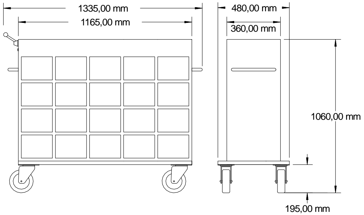
Tipbox trolley 20 ; boxes (double sided ; 40 boxes)
