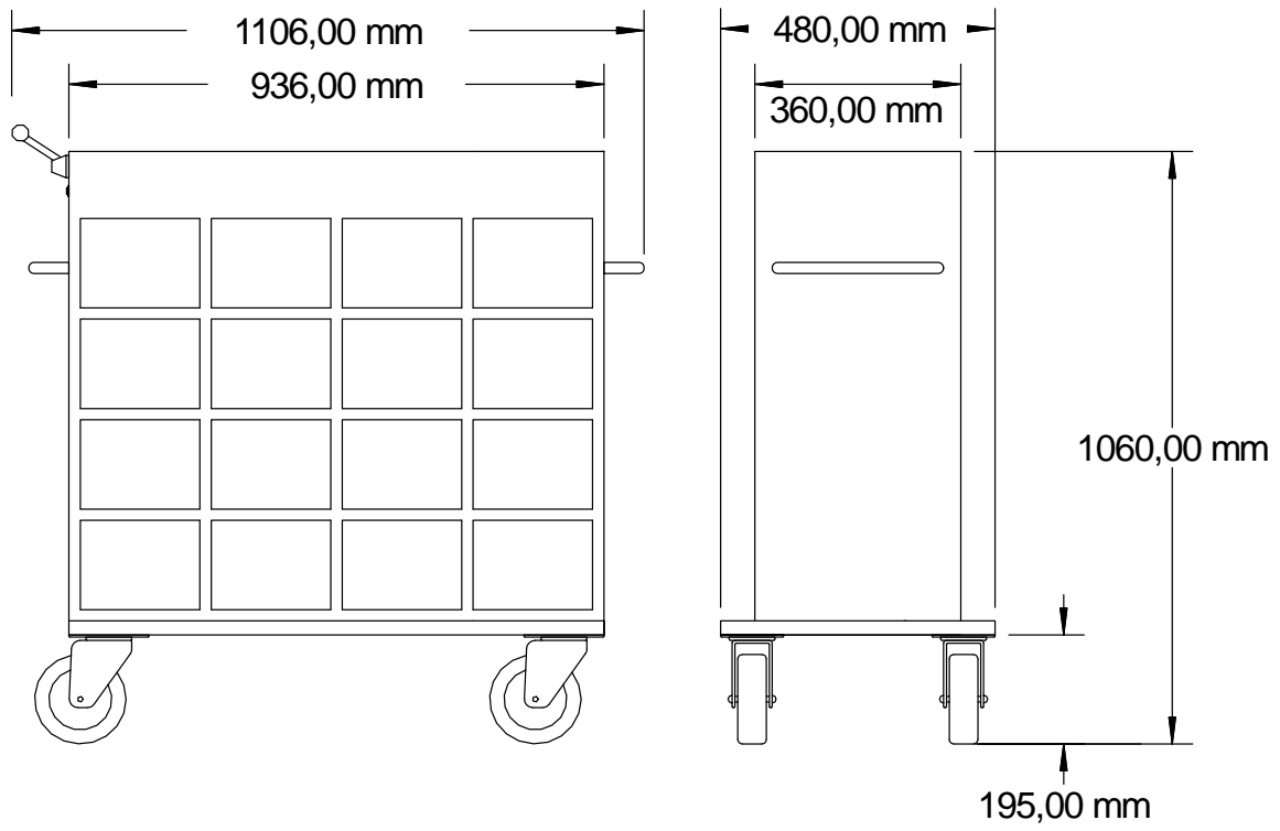
Tipbox trolley ; 16 boxes (double sided ; 32 boxes)
