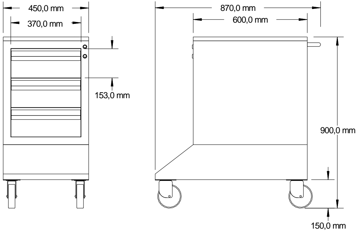
Standard cage trolley 3 drawers
