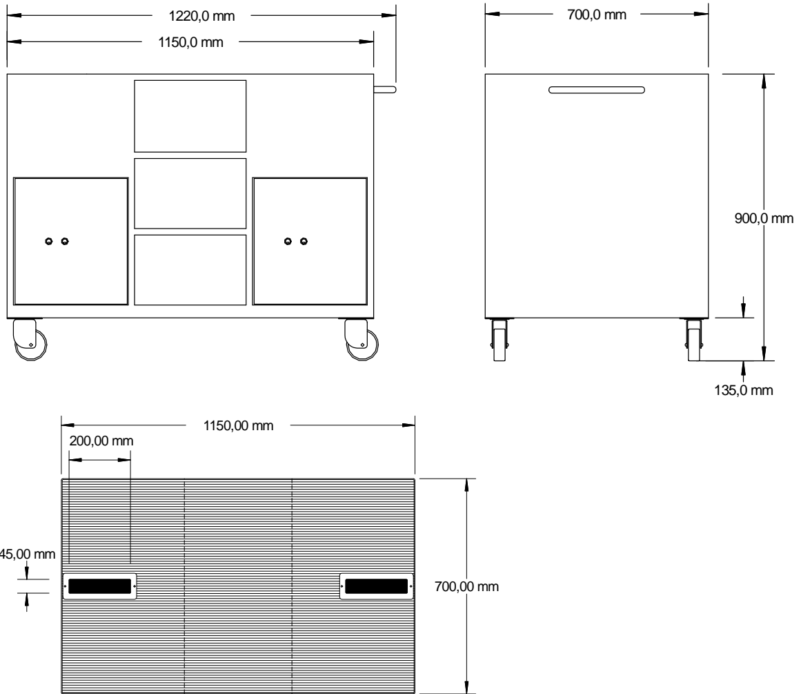
Sealbag trolley, 2 containers, 3 shelves
