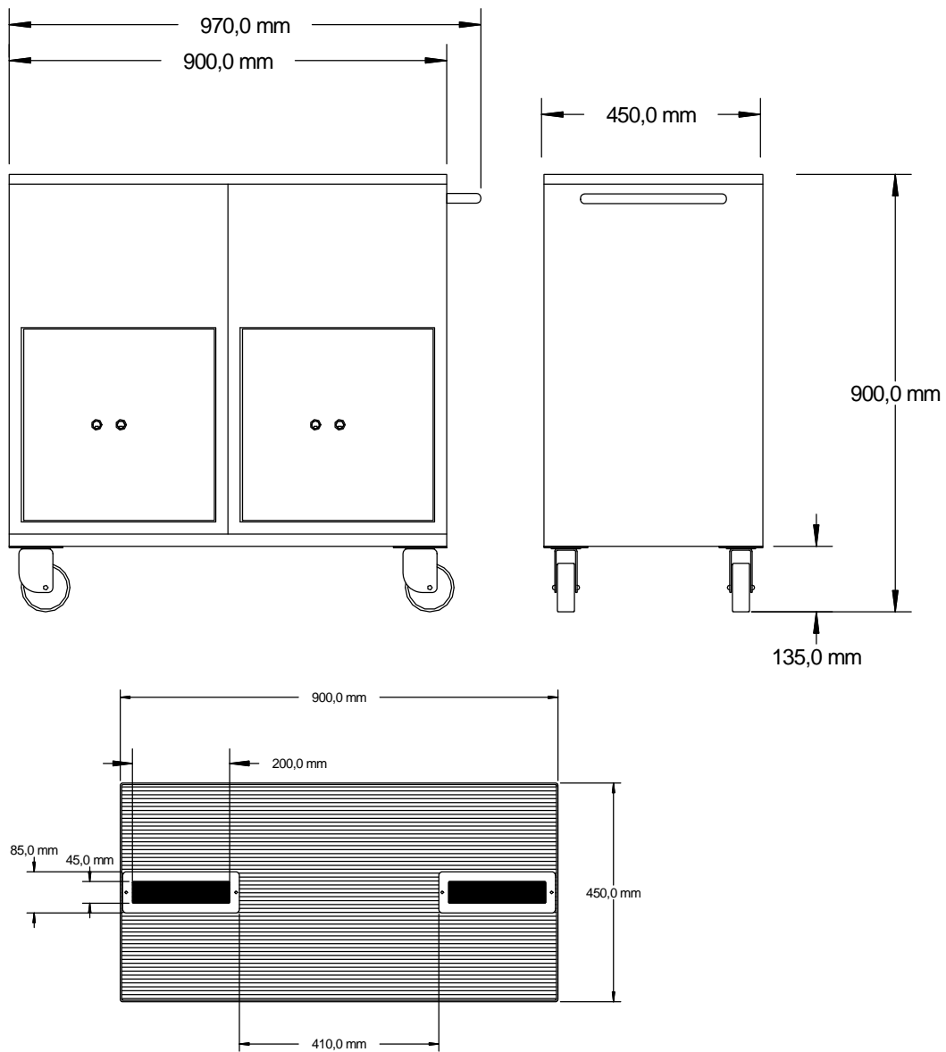
Sealbag trolley, 2 containers
