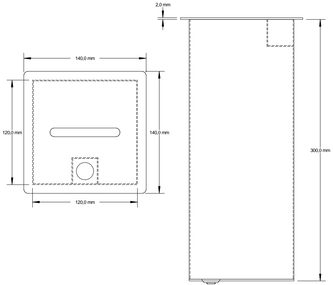
Tipbox 120 x120 x 300 mm with lifting hole/chamber
