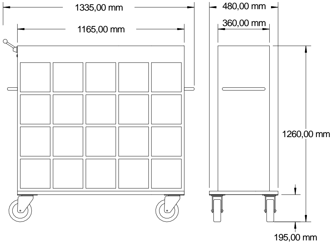
Cashbox trolley ; 20 boxes
